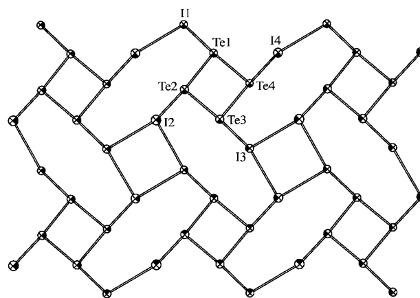
Figure 3. The crystal packing of 1 illustrating the long-range I⋯I contacts linking the structure into small (Te 4 ) and large squares (I 4 ), d(\text{I–I}) = 3.841(3)–3.898(3) Å; phenyl rings are omitted for clarity.
